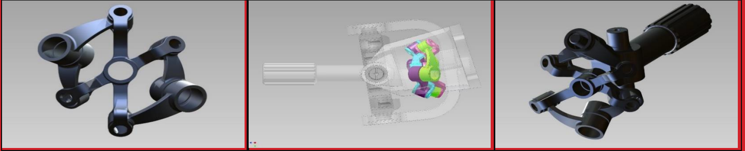
Graphic of the Thompson Coupling showing the internationally patented, spherical 4-bar linkage centring mechanism.
